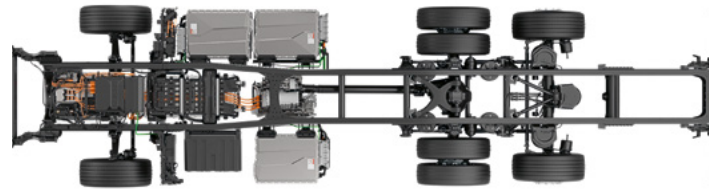
5 battery packs
