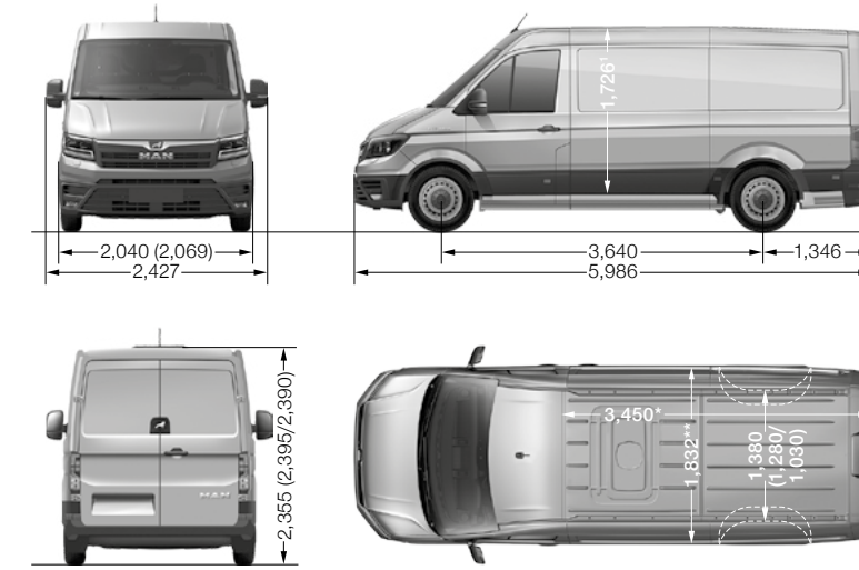
MAN TGE standard panel van with normal roof
