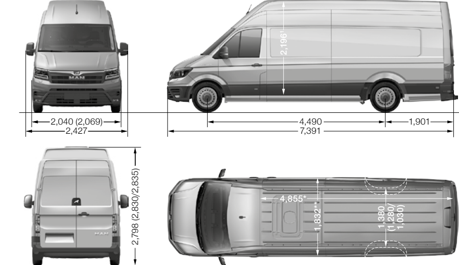
MAN TGE extra-long panel van with super-high roof
